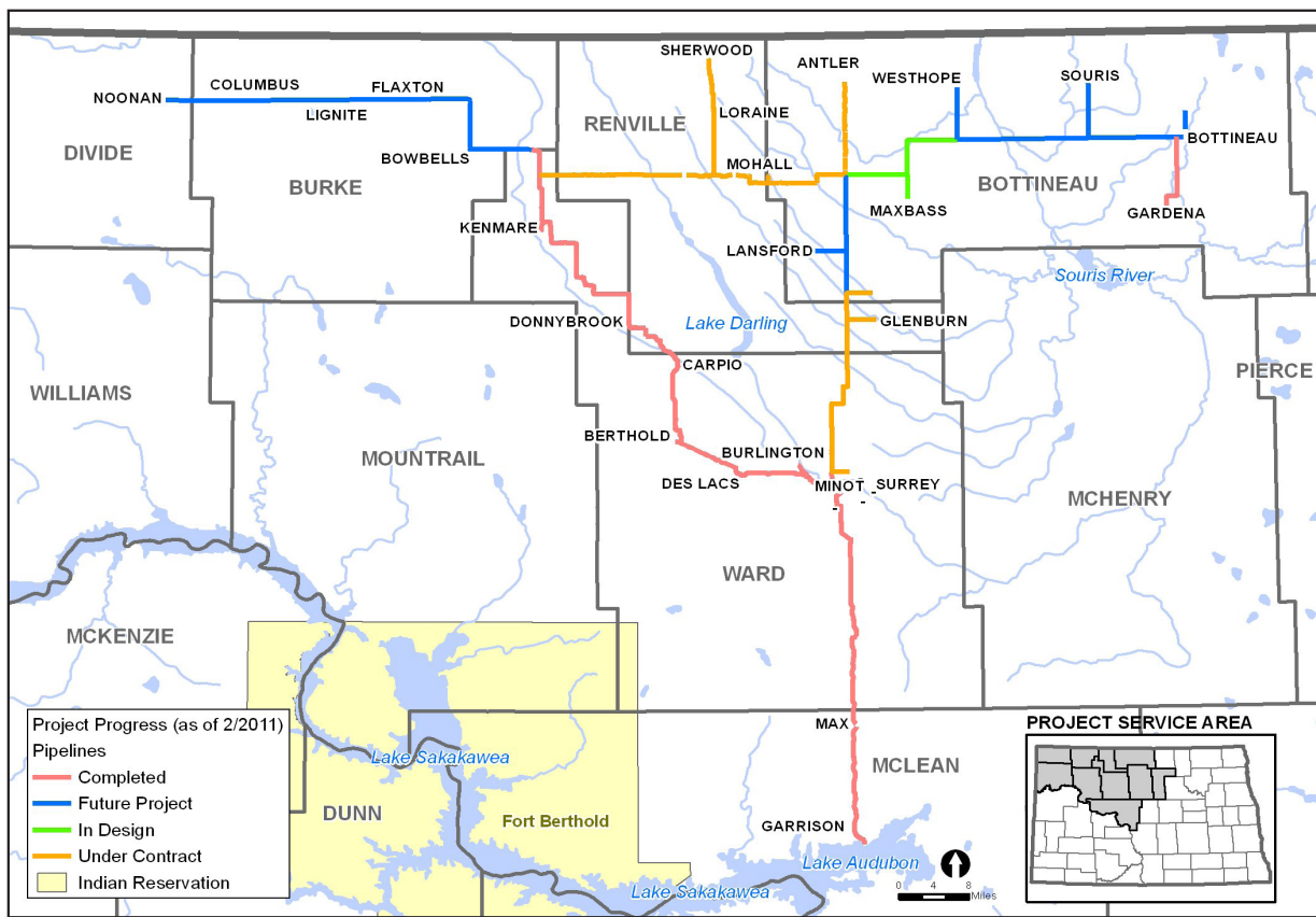
Northwest Area Water Supply project service area.
